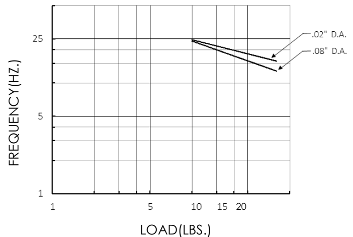
Figure 1: Load Vs. Frequency
