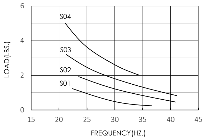
Figure 2: Load Vs. Frequency
