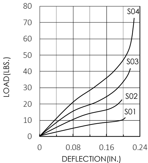
Figure 1: Load Vs. Deflection
