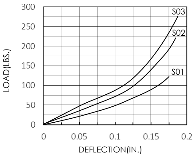
Figure 1: Load Vs. Deflection
