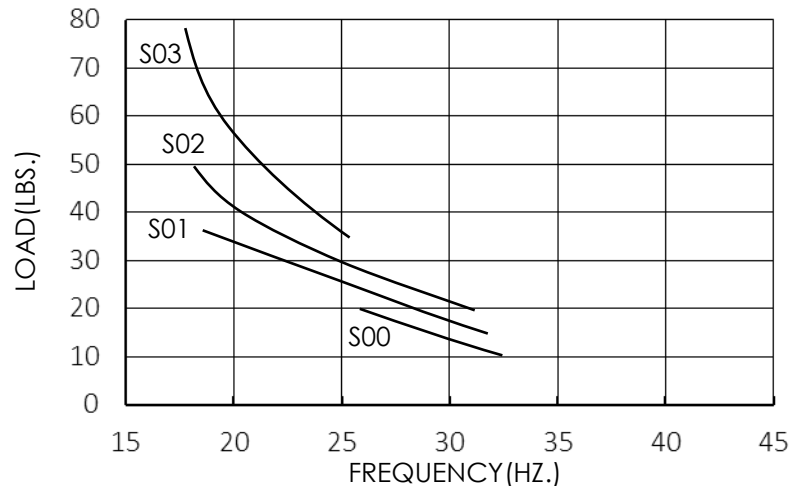
Figure 2: Load Vs. Frequency
