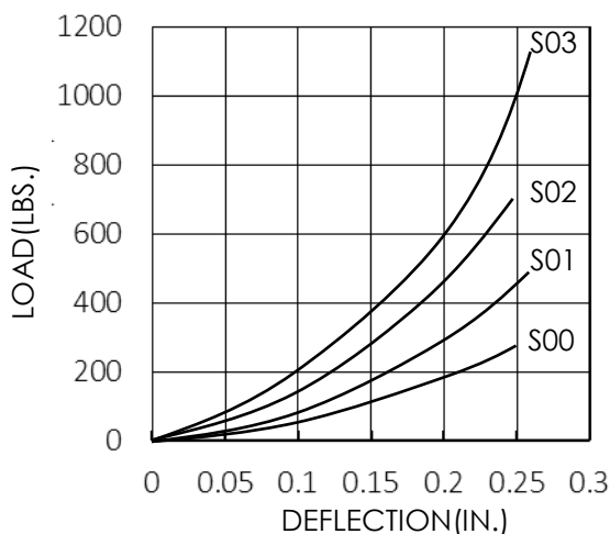
Figure 1: Load Vs. Deflection
