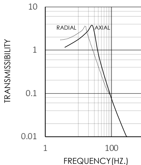
Figure 1: Transmissibility Curve
